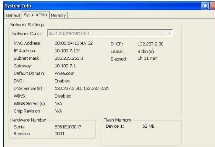
Figure 31 System Info - System Info tab
